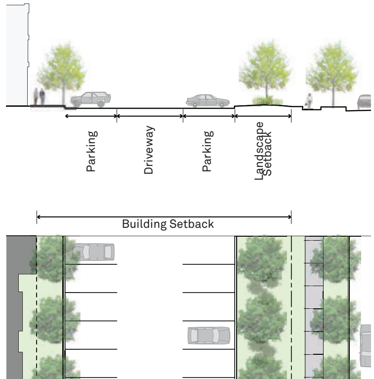
Sample surface parking plan for Employment/Industrial buildings.
